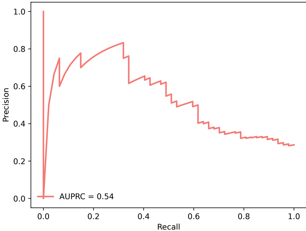
SVM Precision-Recall Curve
